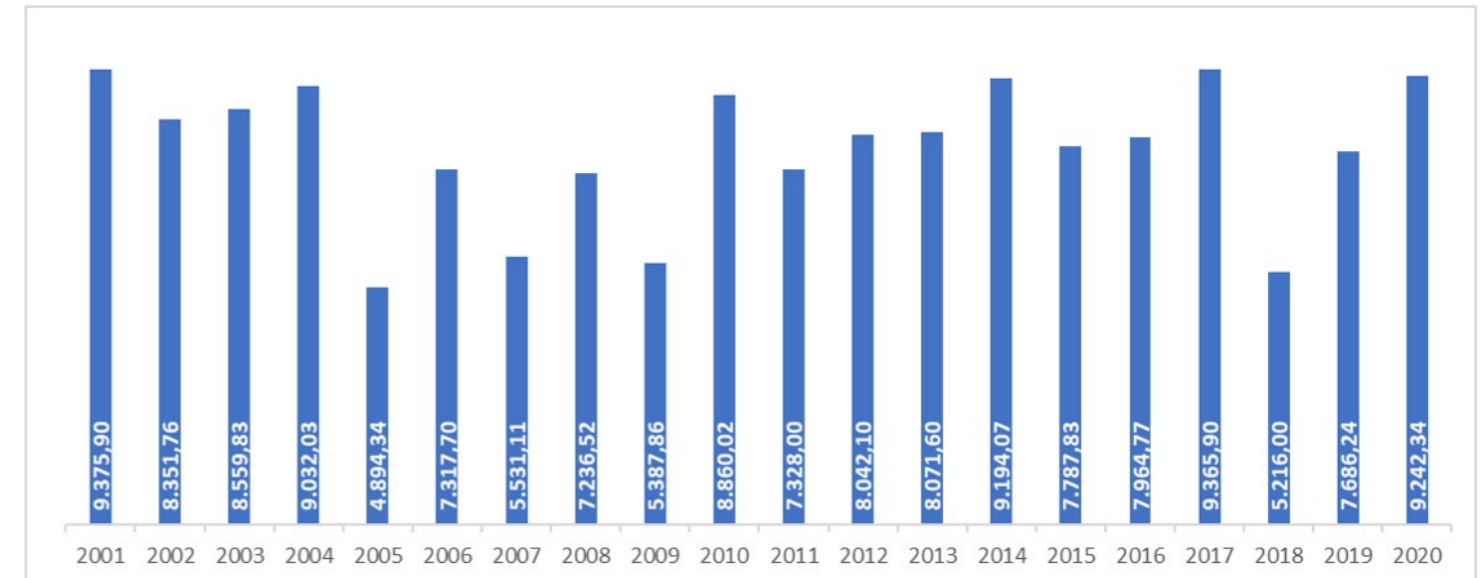
VANDELLÓS II NPP GROSS ELECTRIC POWER PRODUCTION (GWh)
